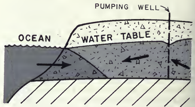
CONTROLLED PUMPING
