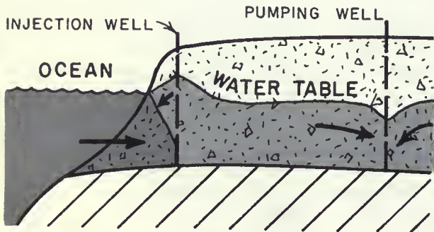
INJECTION BARRIER
