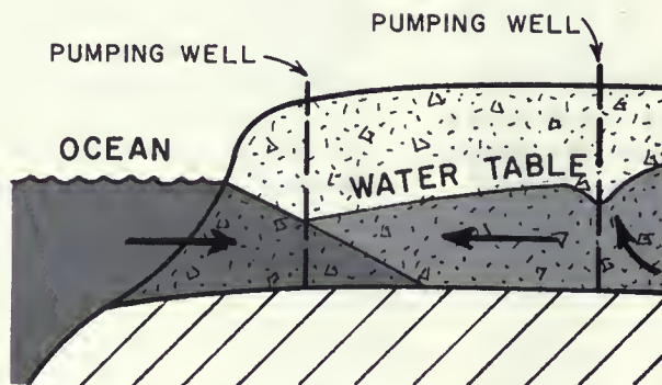
PUMPING TROUGH BARRIER
