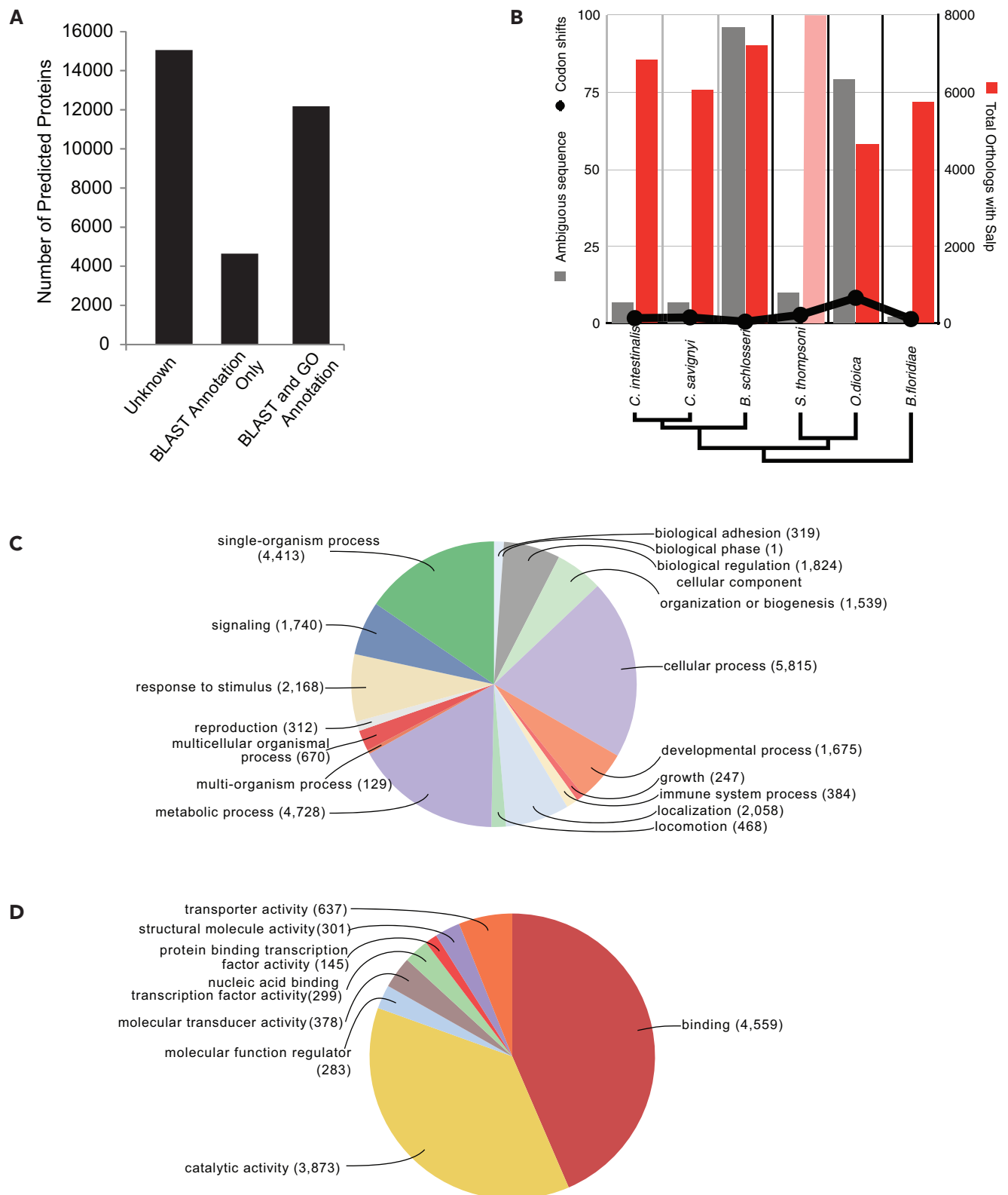
Fig. 2. — Salpa thompsoni gene annotations. (A) Annotation status of S. thompsoni predicted proteins delineated by validation method. (B) The number of ambiguous sequences, codon shifts (left) and total orthologues (right) with S. thompsoni are shown for each species (bottom). Phylogenetic relationships for each species are indicated. (C and D) Pie chart summary of level 2 gene ontology terms associated with biological process (C) and molecular function (D) categories for all annotated S. thompsoni predicted proteins.
